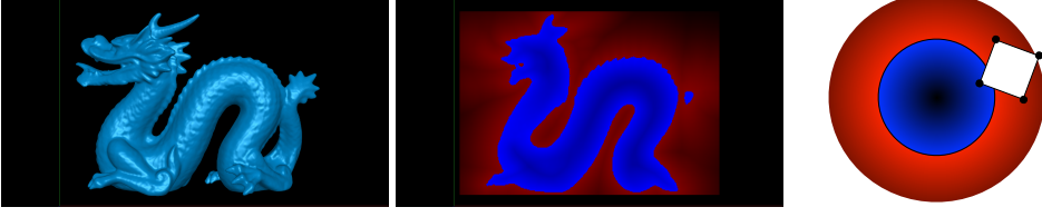
Fig. 12. Left and middle: Three-dimensional dragon model and two-dimensional slice of its signed distance field. Right: Signed distance field for a circle. The vertices of a polygonal shape, illustrated in white, can be efficiently tested against the signed distance field to detect the interpenetration.
