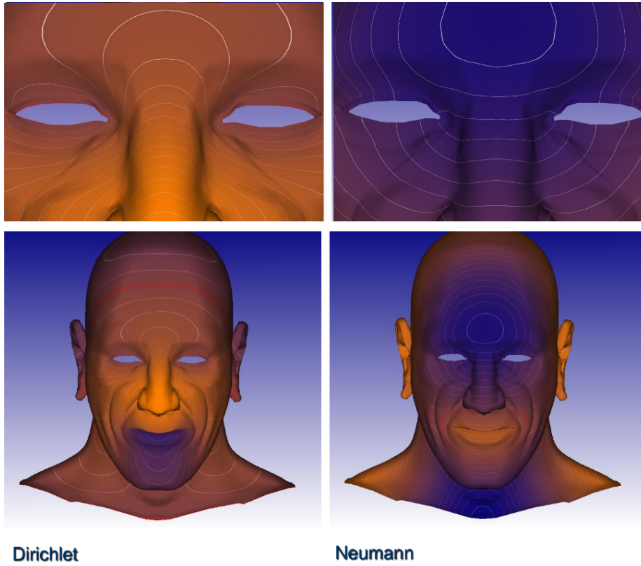
Figure 17: Contour lines of eigenfunctions obtained with Dirichlet boundary conditions (left) and Neumann boundary conditions (right)
