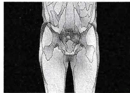
38. Hyperthermia
