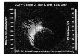
25. Auroral Oval and Earth's Magnetosphere During a Polar Substorm
