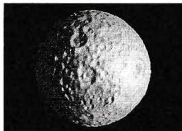
17. Lunar Topography
