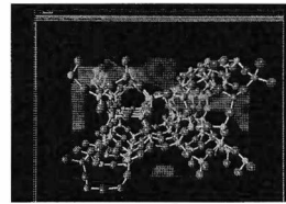
49. Potential energy in a zeolite channel
