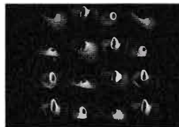
8. Linear superposition of Eigenstates of H
