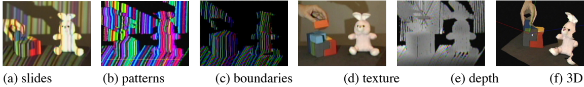
Figure 1: System pipeline.
