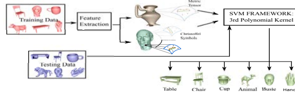
Figure 1: Overview of the 3D object categorization Framework
