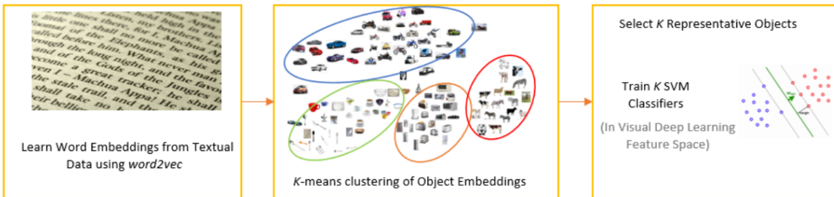
Figure 1: 1. From textual data, learn word embeddings using word2vec . 2. Cluster object embeddings that lets co-occurring objects fall in the same cluster. 3. Select representative object from each cluster that has maximal visual training data. Train visual classifiers for these representative objects. Given a test image, we guess objects (using word embeddings) in the image based on representative objects' detections
