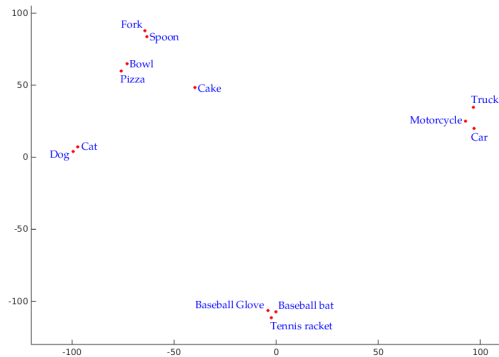
Figure 2: 2-d t-sne [Van Der Mateen and Hinton 2008] projection of word embeddings of objects.
