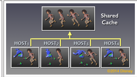
Fig 3: Parade distributes caching to hosts
