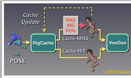
Fig 2: RigCache queries geometry cache for pose
