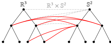
Figure 2: Double hierarchy for the product space.
