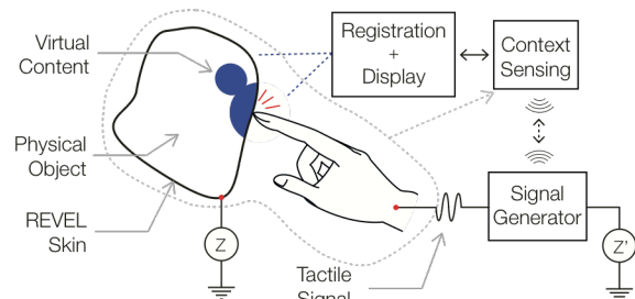
Figure 3: REVEL tactile AR system diagram.
