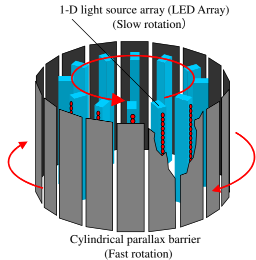
Figure 1: Schematic diagram of basic structure
